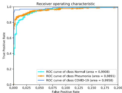
Fig. 8. ROC curves of EDL-COVID prediction on COVIDx test dataset with respect to each class type.
