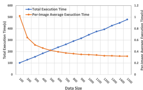
Fig. 9. Execution time for EDL-COVID under different numbers of testing CXR images.
